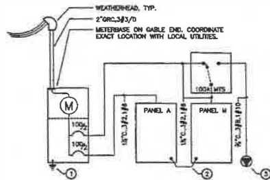
1 ELECTRICAL SINGLE LINE DIAGRAM SCALE: NTS
