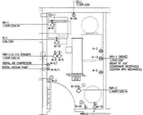
2 ENLARGED MECHANICAL ROOM - POWER E3.1 SCALE: 1/2" = 1'-0"
